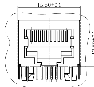
RECOMMENDED PANEL CUTOUT AND JACK LOCATION
